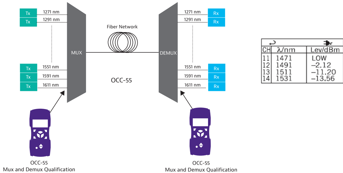
Figure 7. Mux and demux verification with the OCC-55
