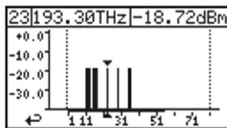
Figure 6. Transmitter wavelength and output power measurement with the OCC-55
