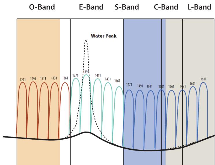
Figure 1. CWDM channel allocation according to ITU-T G.694.2 wavelength grid
